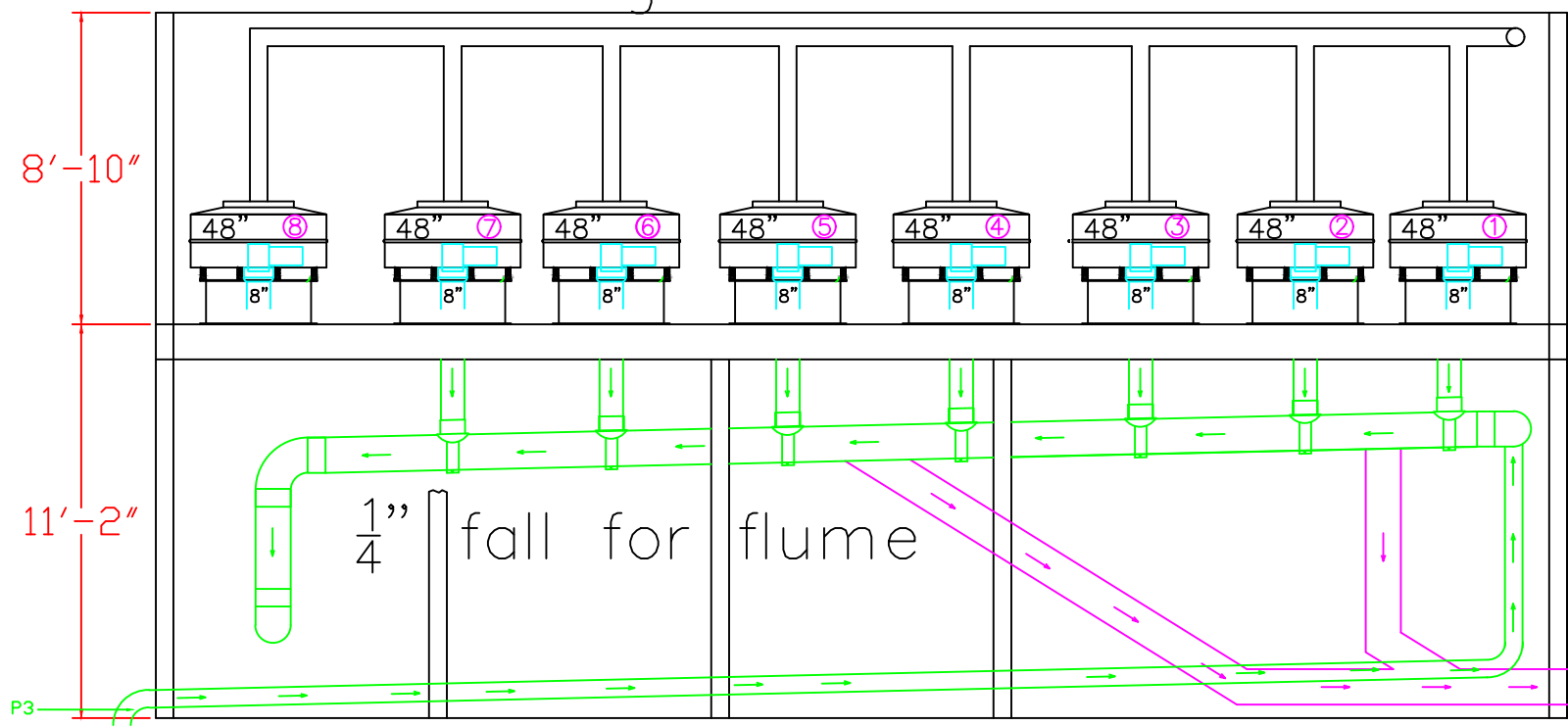
Layout existing 7 vibe screens New flume with feed piping
