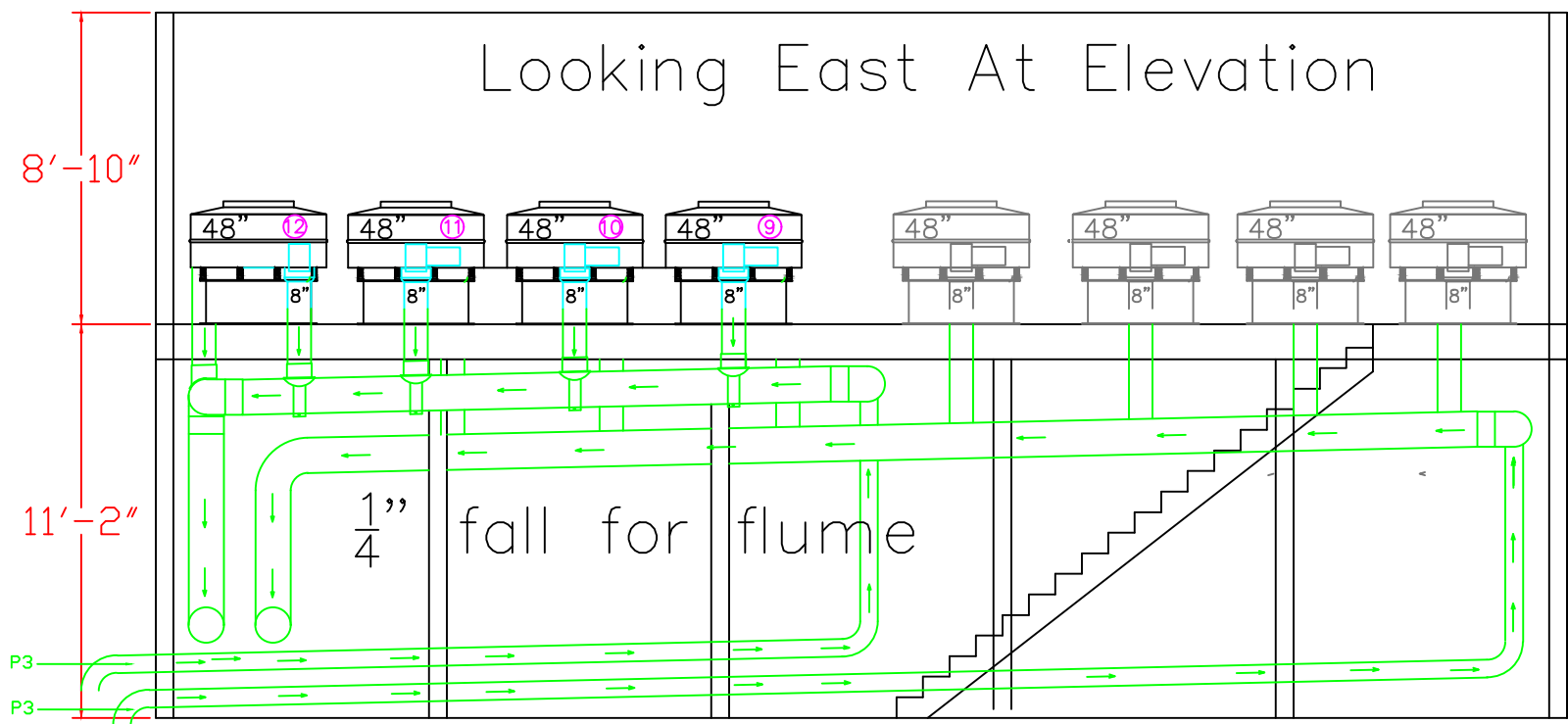
Layout for new vibe screens plus flume with feed piping
