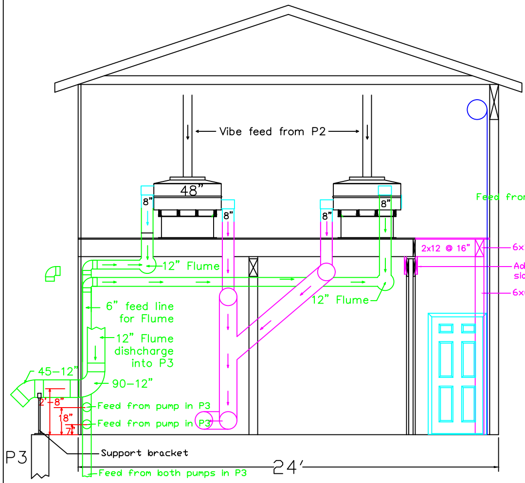
North Elevation
